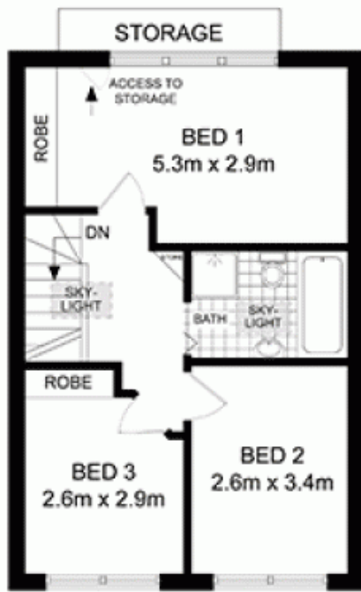
UPPER LEVEL
