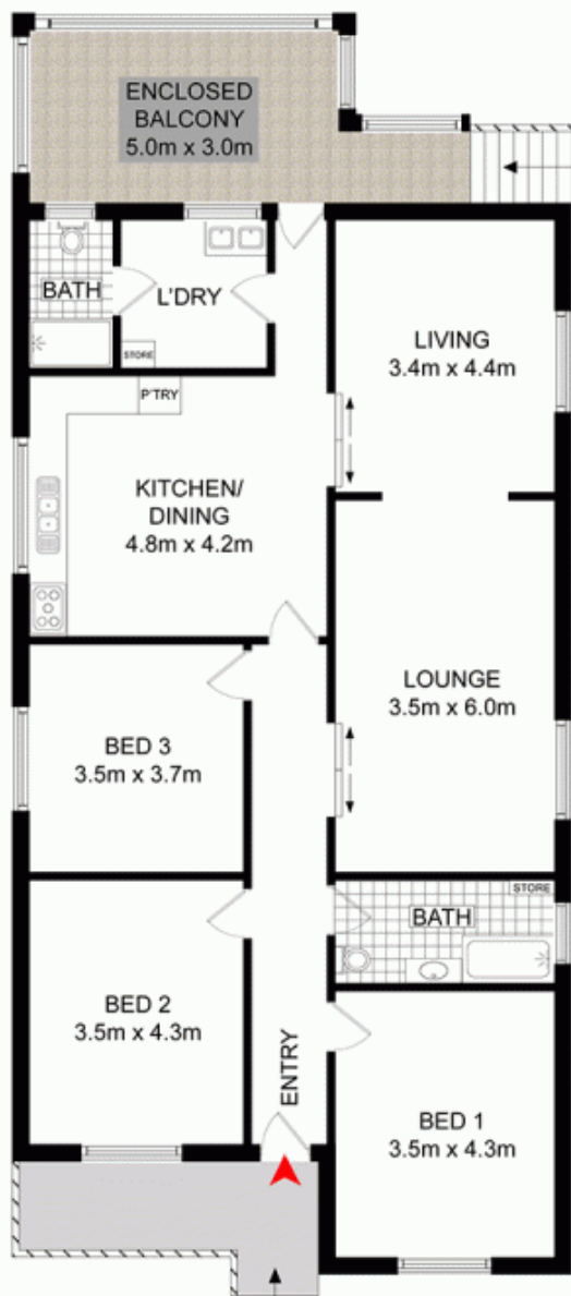
GROUND FLOOR
