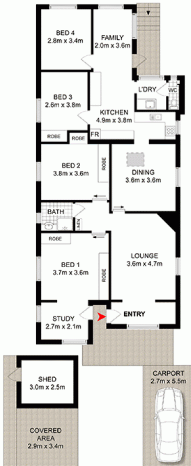
GROUND FLOOR
